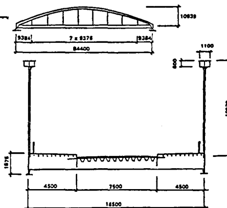
Fig. 2b. Tied arch bridge K 138
