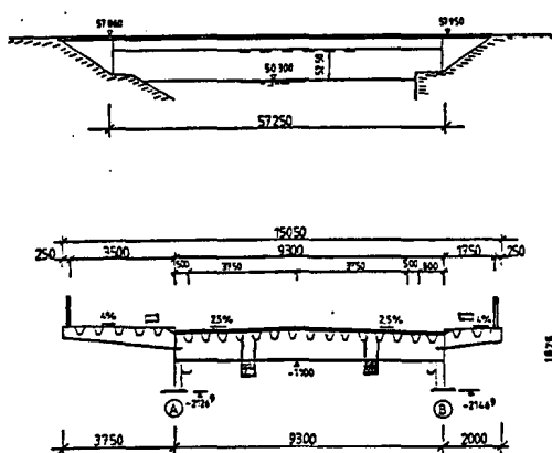
Fig. 2a. Single span bridge K 210
