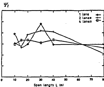
Fig. 5 : \Psi_1 values for bridge elements
