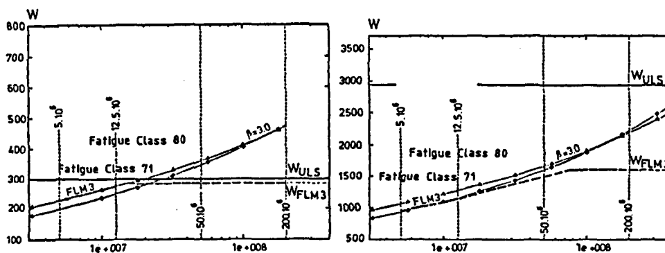
Fig. 6a. W_{required} - Main girder, L = 20 m Fig. 6b. W_{required} - Main girder, L = 80 m
