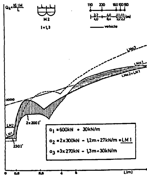
Fig. 8b. Target values - M_2 - Local effects
