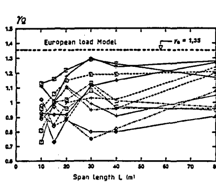
Fig. 4 : \gamma_Q values for bridge elements
